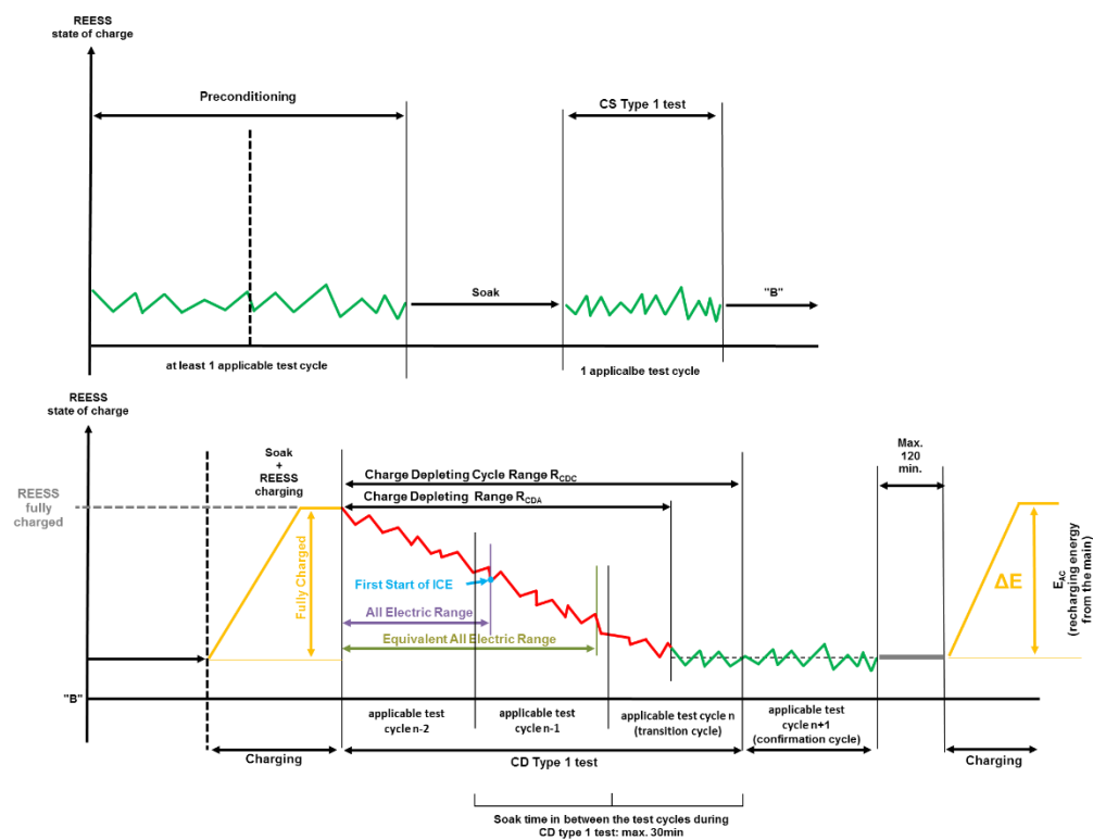
Figure A8.App1/4 OVC-HEVs, charge-sustaining Type 1 test with subsequent charge-depleting Type 1 test'
